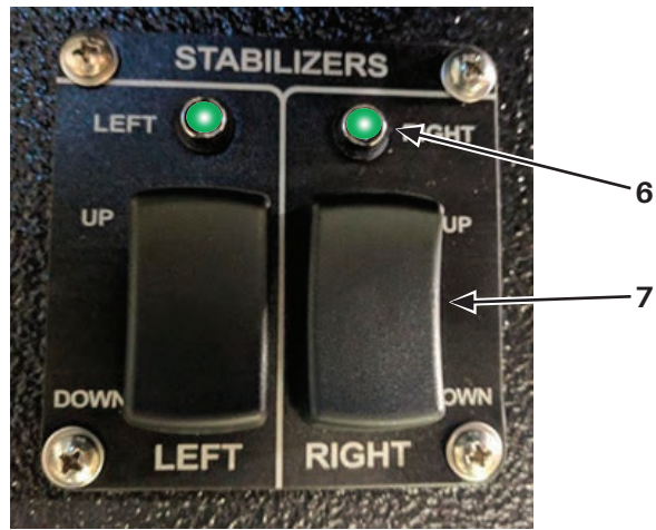
Figure 3-3. Center Stabilizer Controls and Deployed Indicator Lights
