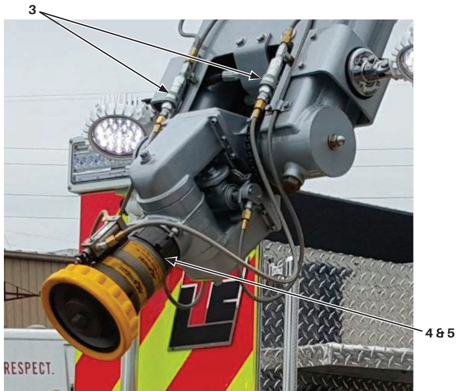
Figure 4-3. Nozzle Coupling & Quick Connects
