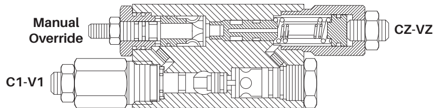
Figure 5-2. Holding valve
