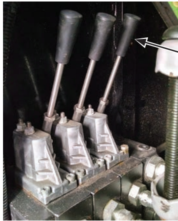
Figure 4-5. Manually Overriding the Sqrt Electric Controls
