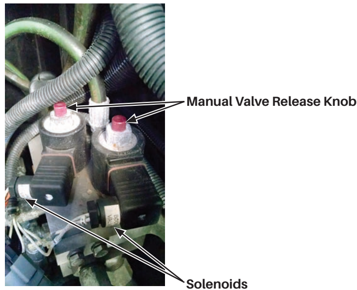
Figure 4-4. Overriding the Diverter Valve Electrical Controls
