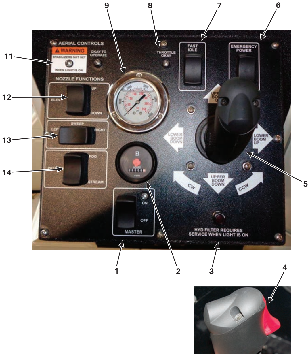
Figure 3-5. Primary Operator control station
