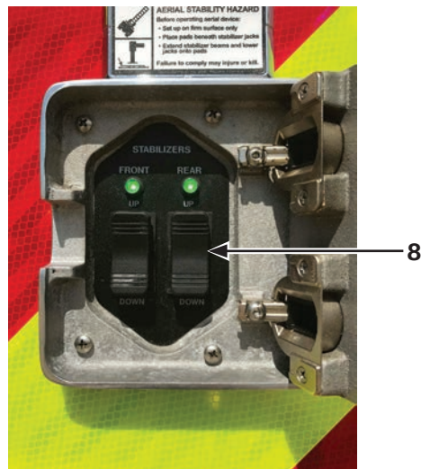
Figure 3-4. Stabilizer individual controls
